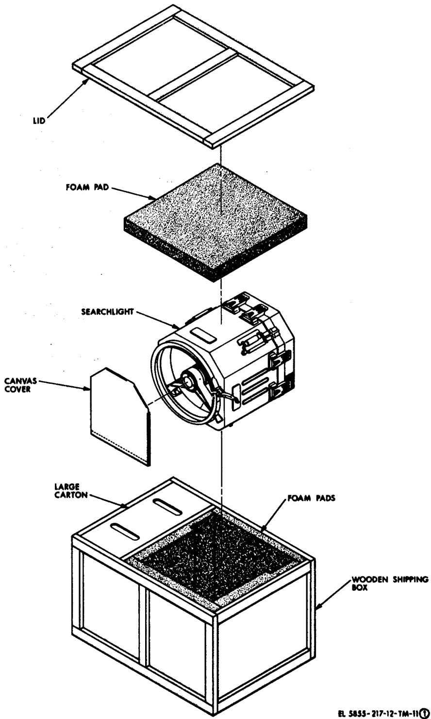
Figure 8-1①. Typical packaging of the searchlight set (part 1 of 2).
